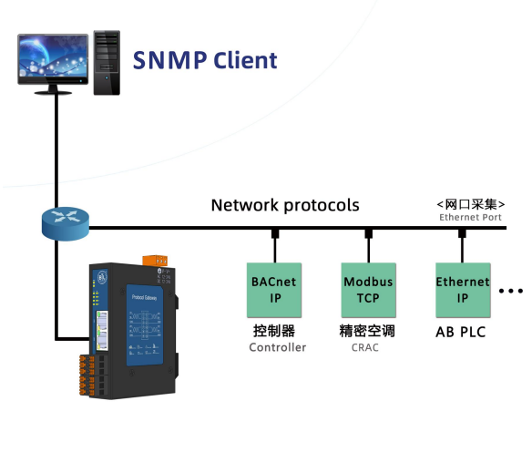
场景1：集成网口协议到SNMP Client Application-1: Integrate the network port protocol to SNMP Client
