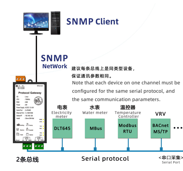
场景2：集成串口协议到SNMP Client Application-2: Integrate the serial port protocol to SNMP Client
